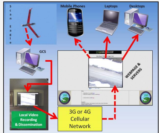
Flow diagram of video streaming from the ScanEagle UAS during deployments (dashed lines are wireless links).
